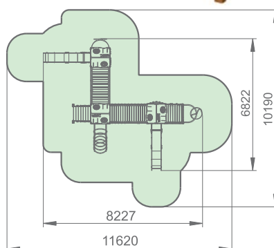
Playground complex «Castle-NEW»
