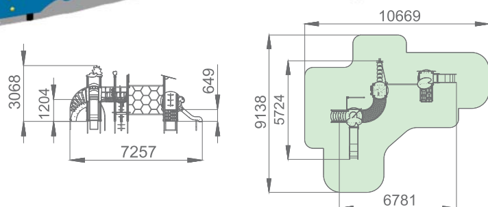
Playground complex «Steamlet-3»
