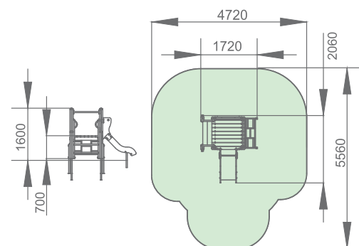
Playground complex «Champion-1»
