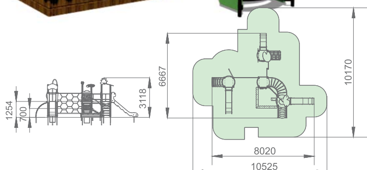
Playground complex «Steamlet-4»
