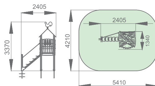
Playground complex «Hatka»
